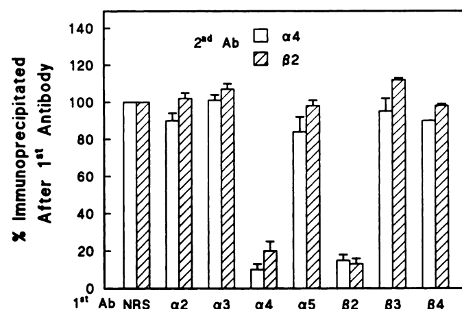
Fig. 8. Association of \alpha 4 and \beta 2 subunits in neuronal nicotinic receptors. Aliquots of [ ^3\text{H} ]cytisine-bound solubilized rat forebrain, equivalent to 20 mg of original weight, were incubated for 4 hr at 4° with either NRS, anti- \alpha 2 , - \alpha 3 , - \alpha 4 , - \alpha 5 , - \beta 2 , - \beta 3 , or - \beta 4 serum (1 st Ab). After precipitation with stripped PANSORBIN, supernatants were incubated for an additional 4 hr with a second antibody (2 nd Ab), either anti- \alpha 4 serum ( \square ) or anti- \beta 2 serum ( \blacksquare ). Nonspecific immunoprecipitation was determined with NRS. Data from four experiments are expressed as the mean \pm standard error in dpm/20 mg of tissue.
