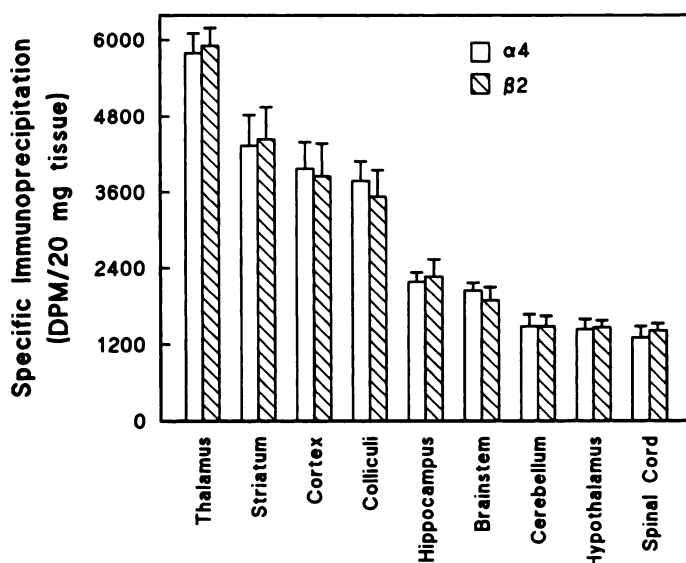
Fig. 7. Regional distribution of neuronal nicotinic receptors containing \alpha 4 and \beta 2 subunits. Homogenates from the indicated rat CNS regions were incubated with [ ^3\text{H} ]cytisine and solubilized. Aliquots of solubilized tissue, equivalent to 20 mg of original weight, were incubated for 4 hr at 4° with either anti- \alpha 4 serum ( \square ) or anti- \beta 2 serum ( \blacksquare ). Nonspecific immunoprecipitation was determined with NRS. Data from four experiments are expressed as the mean \pm standard error, in dpm/20 mg of tissue.
