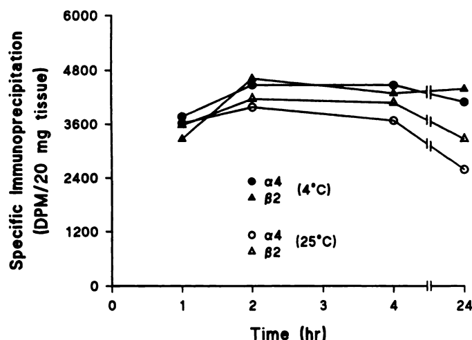
Fig. 1. Time and temperature dependence of the immunoprecipitation of solubilized neuronal nicotinic receptors by anti- \alpha 4 and anti- \beta 2 sera. Aliquots of [ ^3 H]cytisine-bound solubilized rat forebrain, equivalent to 20 mg of original weight, were incubated with either anti- \alpha 4 serum (circles) or anti- \beta 2 serum (triangles) at 4° (closed symbols) or 25° (open symbols), for the indicated lengths of time. Nonspecific immunoprecipitation was determined with NRS. Data are expressed in dpm/20 mg of tissue and are representative of an experiment performed three times.
