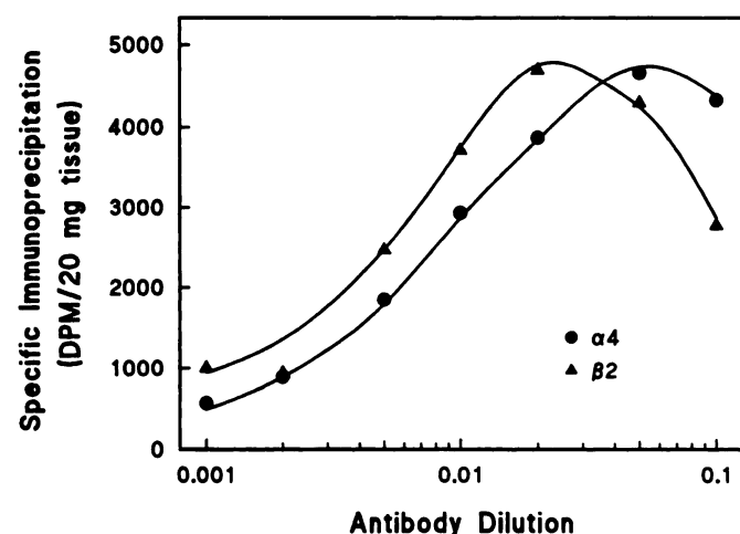
Fig. 2. Anti- \alpha 4 and anti- \beta 2 sera concentration dependence of the immunoprecipitation of solubilized neuronal nicotinic receptors. Aliquots of [ ^3 H]cytisine-bound solubilized rat forebrain, equivalent to 20 mg of original weight, were incubated for 4 hr at 4° with either anti- \alpha 4 serum (●) or anti- \beta 2 serum (▲) at the indicated dilutions. Nonspecific immunoprecipitation was determined with NRS. Data are expressed in dpm/20 mg of tissue and are representative of an experiment performed six times.
