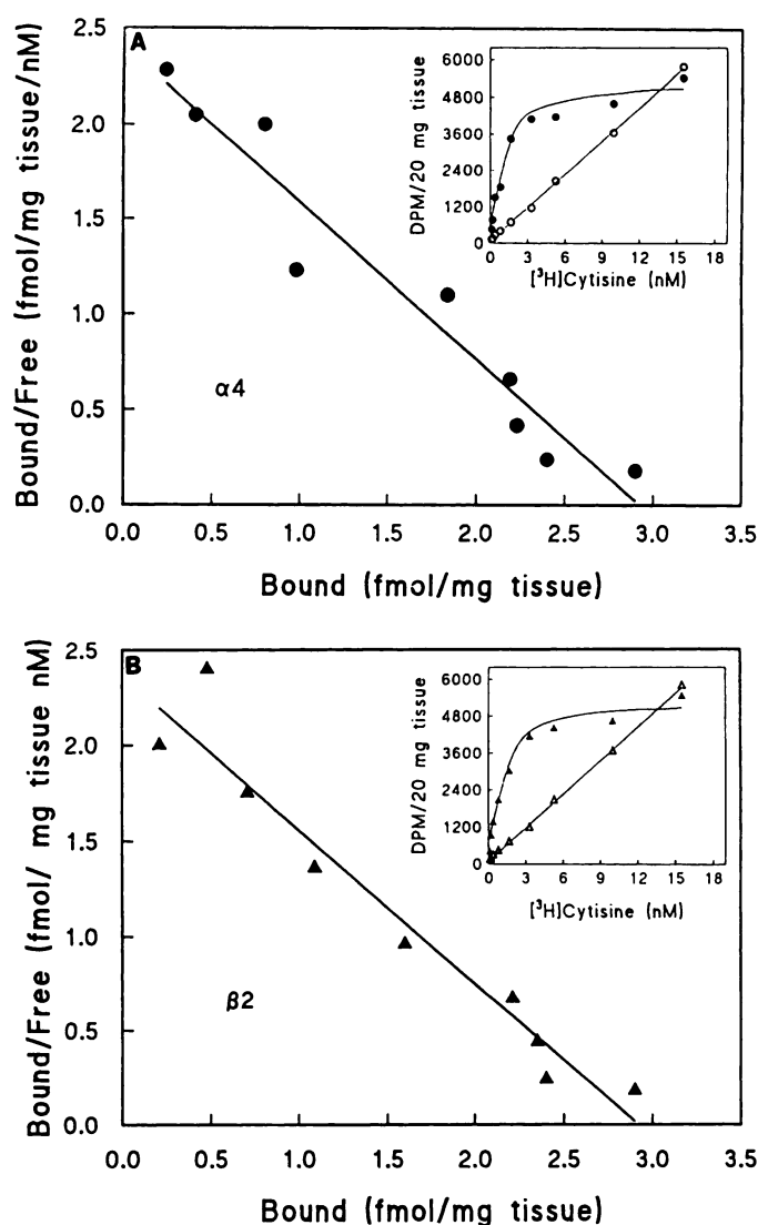
Fig. 6. Saturation analysis of [ ^3\text{H} ]cytisine binding to rat forebrain homogenates immunoprecipitated by anti- \alpha 4 and anti- \beta 2 sera. Rat forebrain homogenates were incubated with 0.15–15 nM [ ^3\text{H} ]cytisine and then solubilized. Aliquots of tissue, equivalent to 20 mg of original weight, were incubated for 4 hr at 4° with antisera. Nonspecific immunoprecipitation was determined with NRS. Scatchard plots depict specific immunoprecipitation by anti- \alpha 4 serum (A) or anti- \beta 2 serum (B); insets, saturation curves depict specific (closed symbols) and nonspecific (open symbols) immunoprecipitation of [ ^3\text{H} ]cytisine-bound receptor. Data are expressed in dpm/20 mg of tissue and are representative of an experiment performed eight times (see Table 1).
